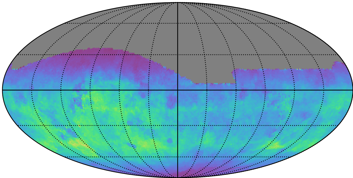
too_elab_r32_d2_giz_v3.4_10yrs All sky g band: Normalized Teff
