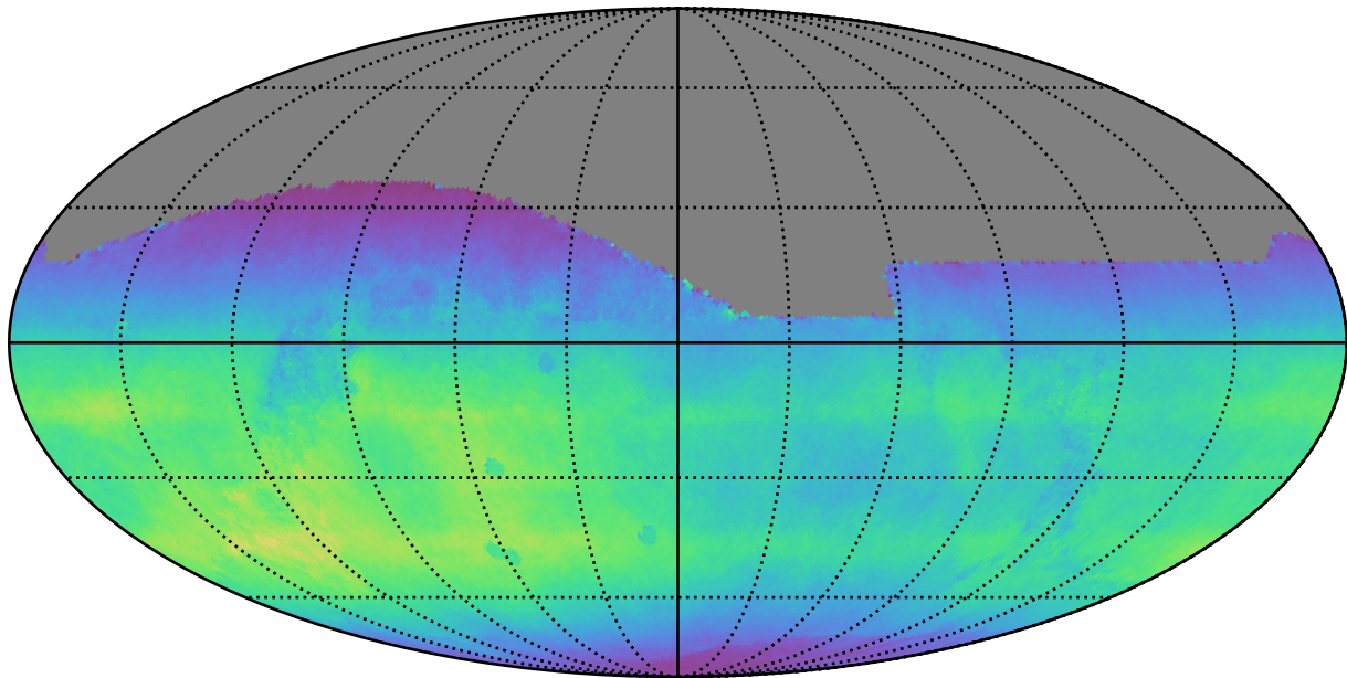
too_elab_r32_d2_giz_v3.4_10yrs All sky all bands: Normalized Teff
