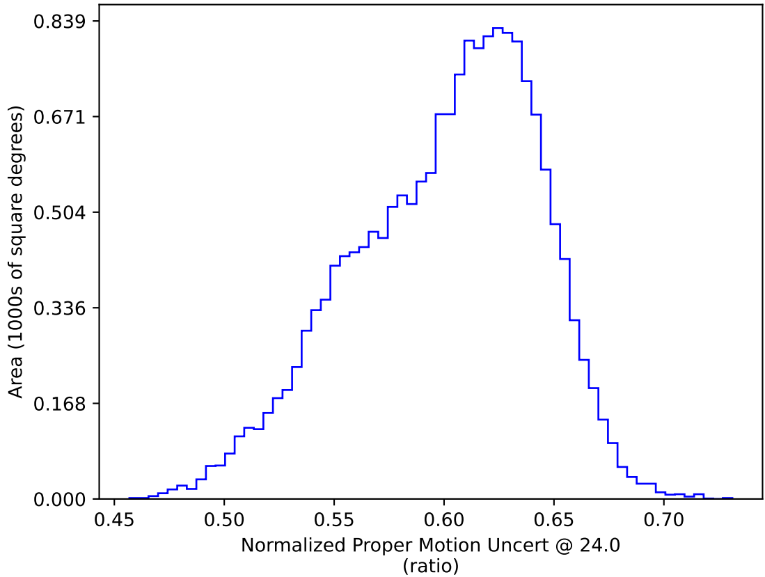
too_elab_r32_d2_giz_v3.4_10yrs WFD: Normalized Proper Motion Uncert @ 24.0
