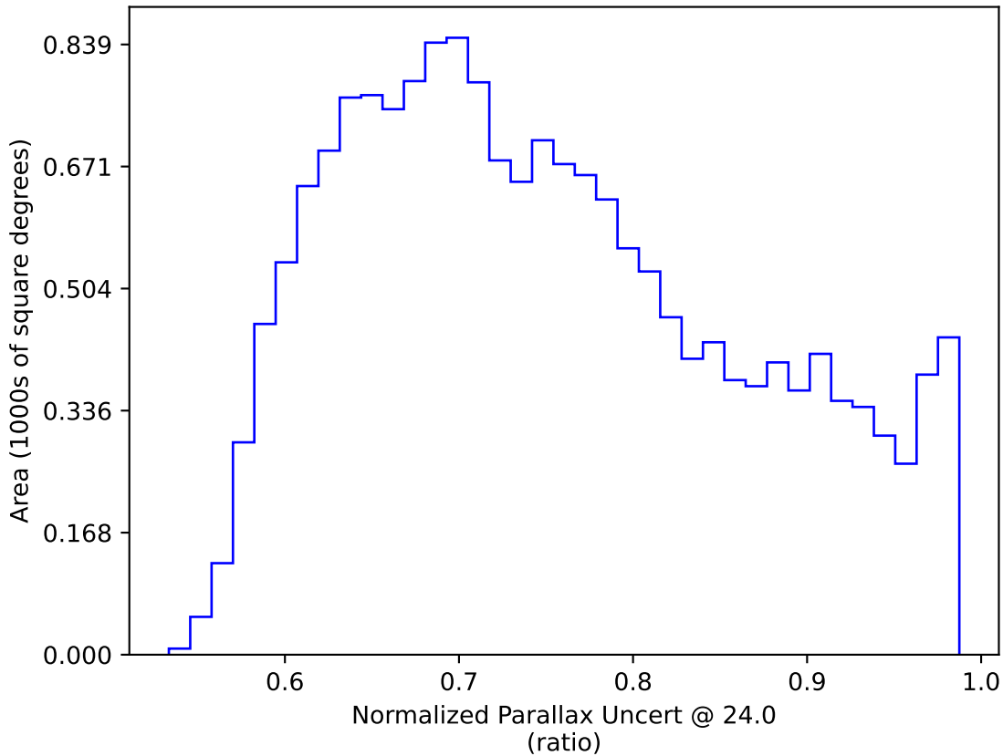
too_elab_r32_d2_giz_v3.4_10yrs WFD: Normalized Parallax Uncert @ 24.0
