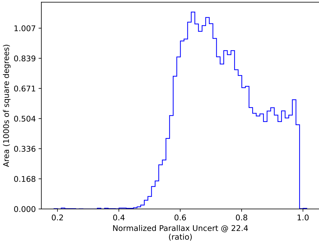
too_elab_r32_d2_giz_v3.4_10yrs All sky: Normalized Parallax Uncert @ 22.4
