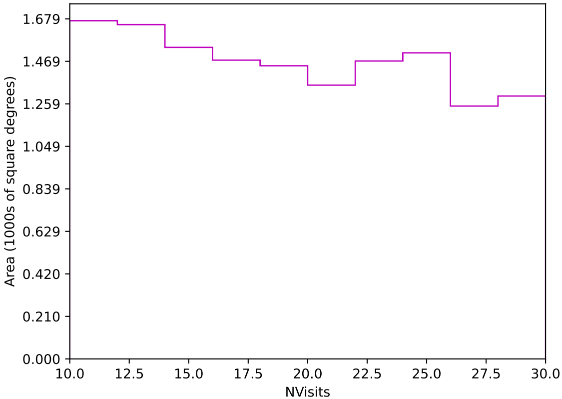
too_elab_r32_d2_giz_v3.4_10yrs Yr 3-4 z band: NVisits
