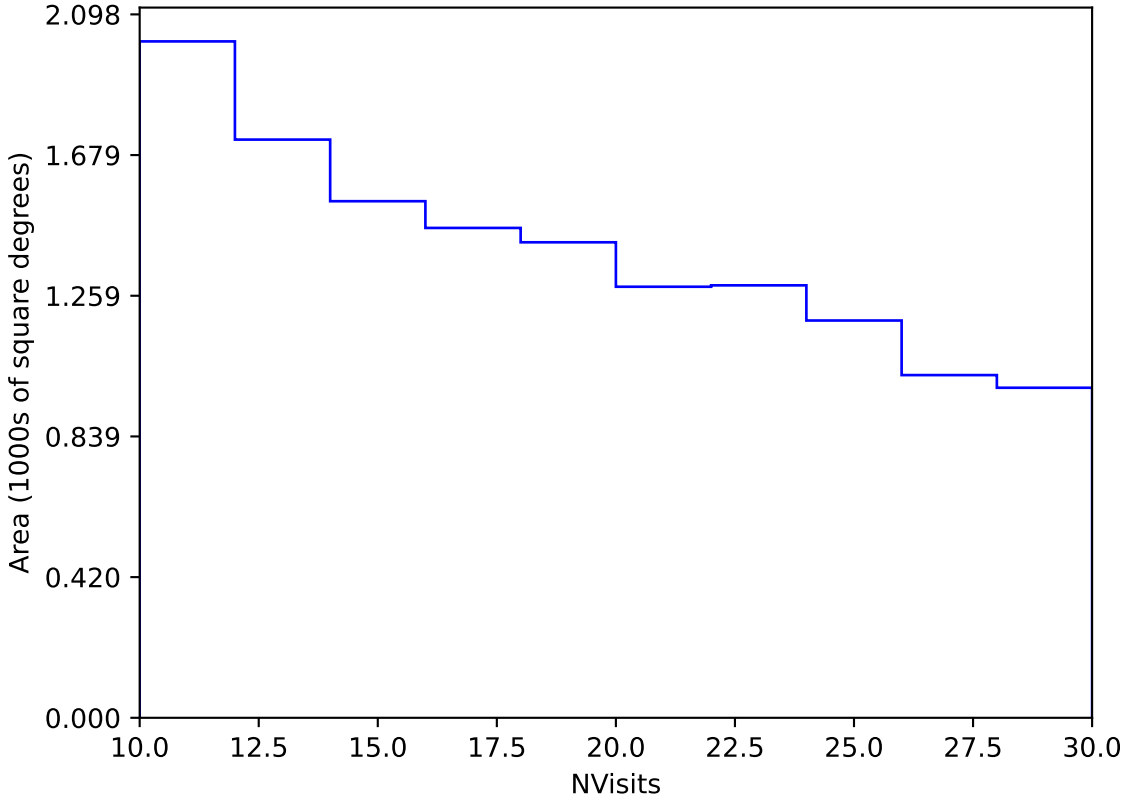
too_elab_r32_d2_giz_v3.4_10yrs Yr 3-4 y band: NVisits
