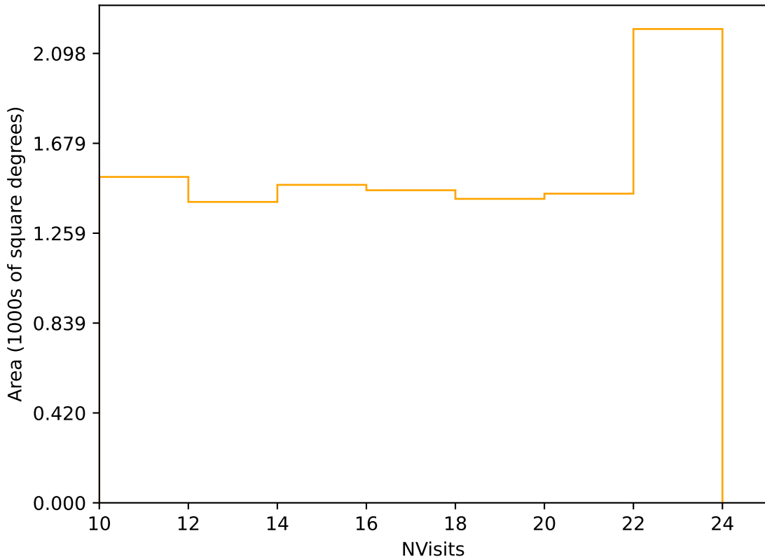
too_elab_r32_d2_giz_v3.4_10yrs Yr 3-4 r band: NVisits
