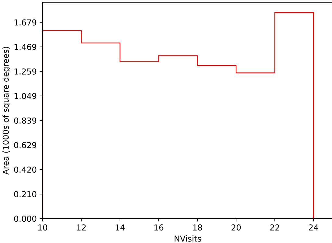
too_elab_r32_d2_giz_v3.4_10yrs Yr 3-4 i band: NVisits
