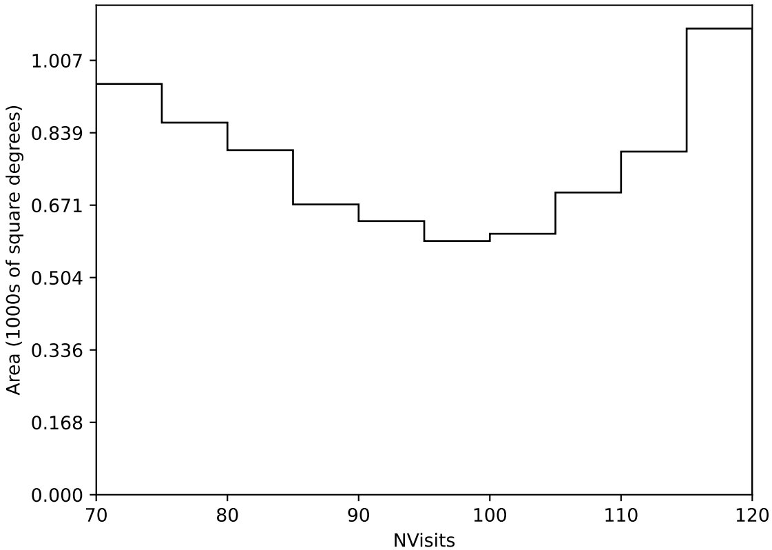
too_elab_r32_d2_giz_v3.4_10yrs Yr 3-4 all bands: NVisits
