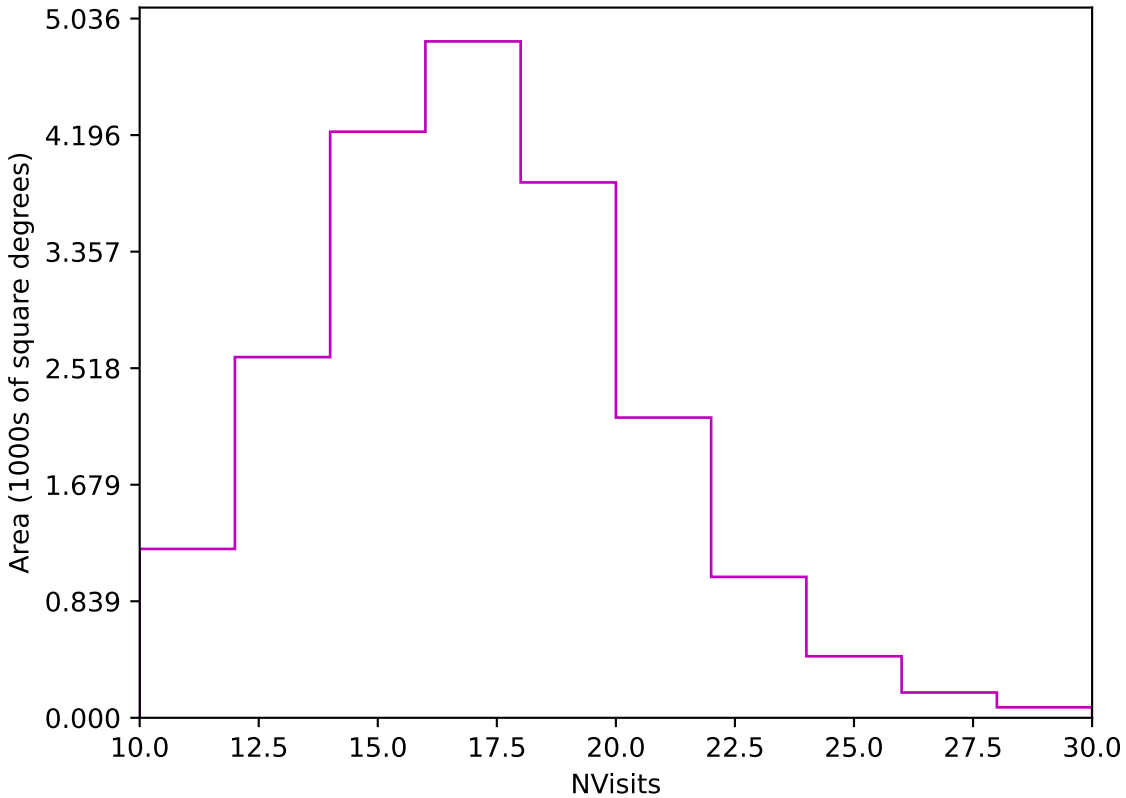
too_elab_r32_d2_giz_v3.4_10yrs Yr 1 z band: NVisits
