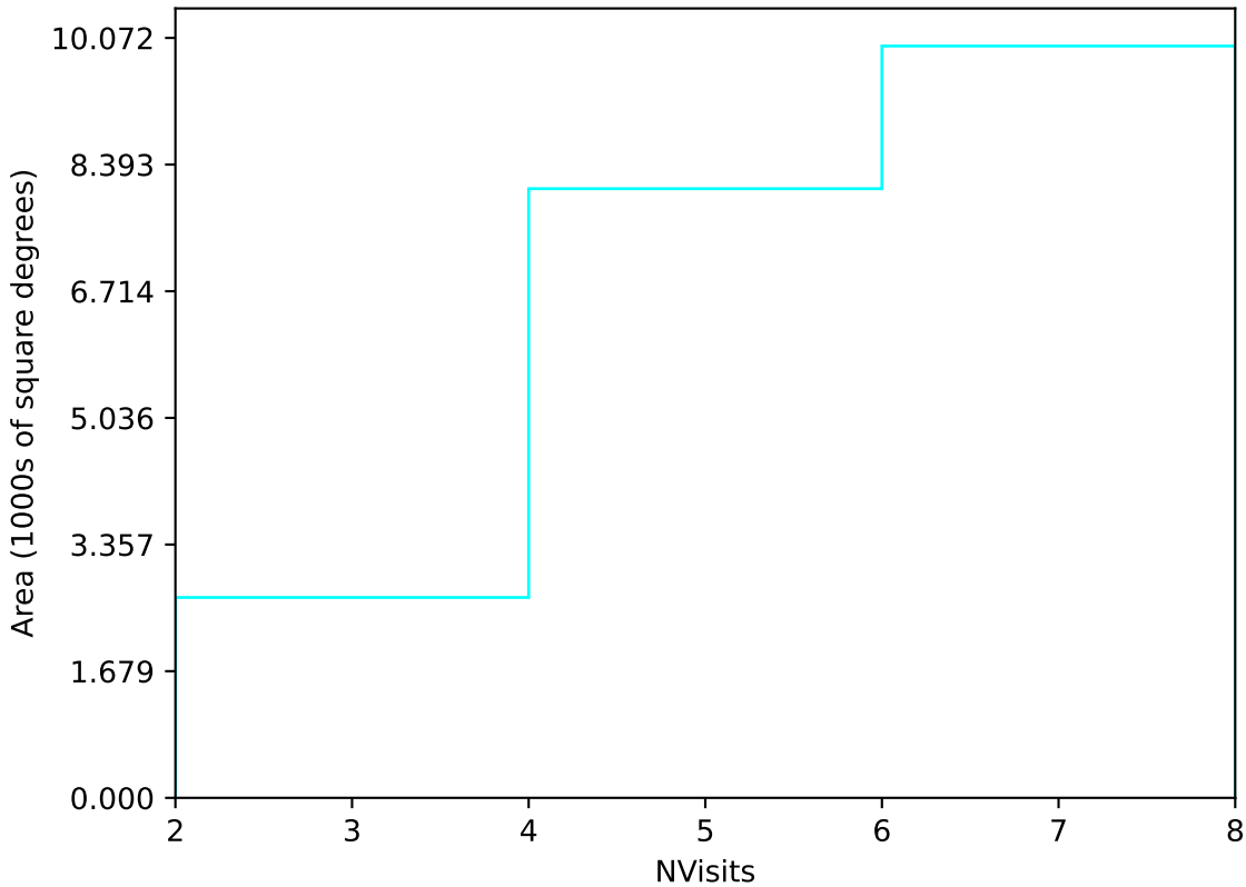
too_elab_r32_d2_giz_v3.4_10yrs Yr 1 u band: NVisits
