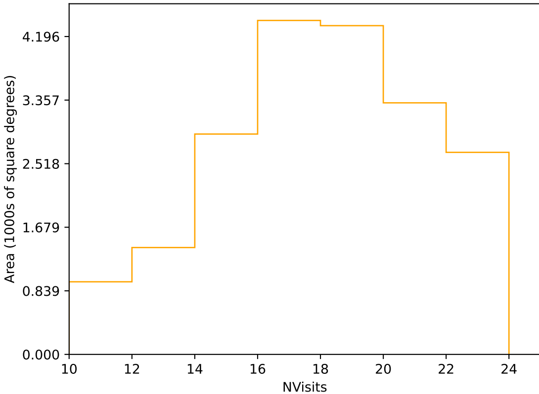
too_elab_r32_d2_giz_v3.4_10yrs Yr 1 r band: NVisits
