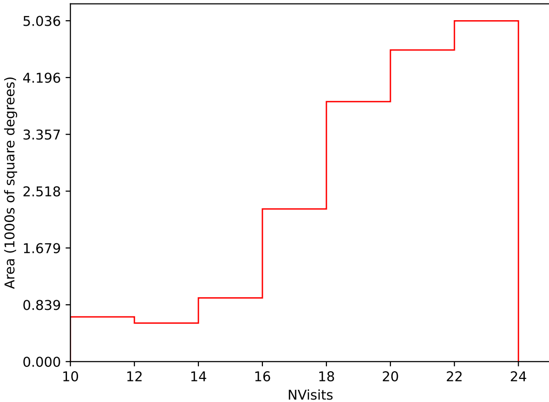
too_elab_r32_d2_giz_v3.4_10yrs Yr 1 i band: NVisits
