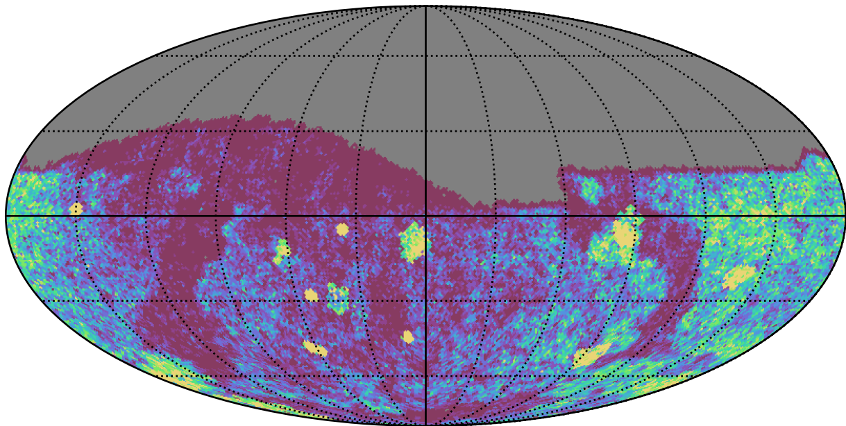
too_elab_r32_d2_giz_v3.4_10yrs Yr 1 g band: NVisits
