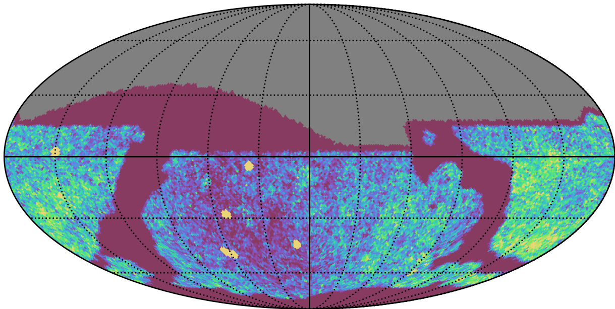
too_elab_r32_d2_giz_v3.4_10yrs Yr 1 all bands: NVisits
