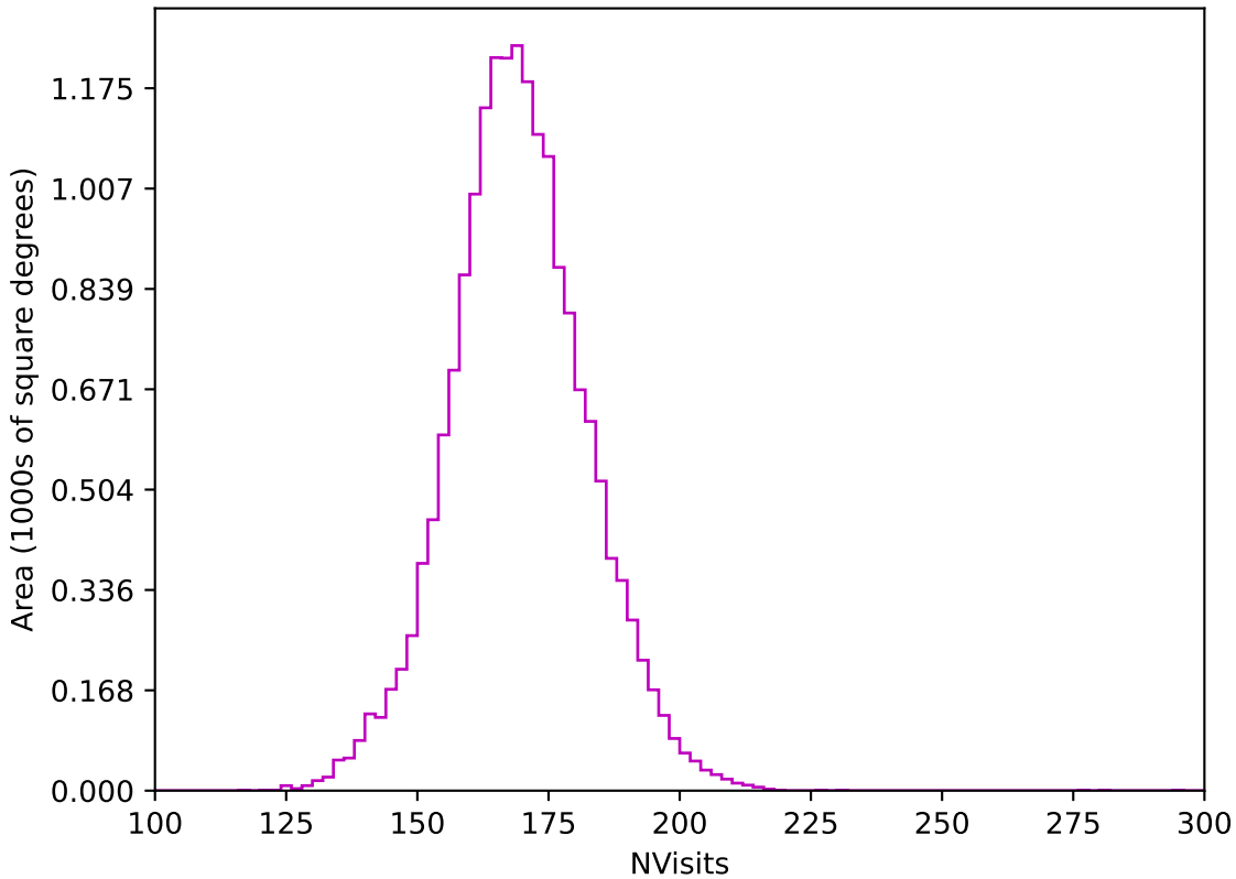
too_elab_r32_d2_giz_v3.4_10yrs WFD z band: NVisits
