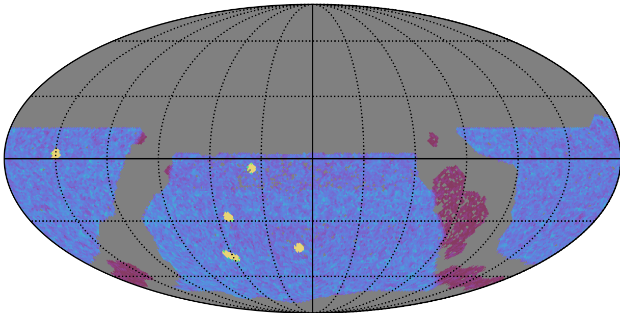
too_elab_r32_d2_giz_v3.4_10yrs WFD y band: NVisits
