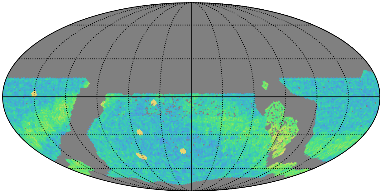
too_elab_r32_d2_giz_v3.4_10yrs WFD r band: NVisits
