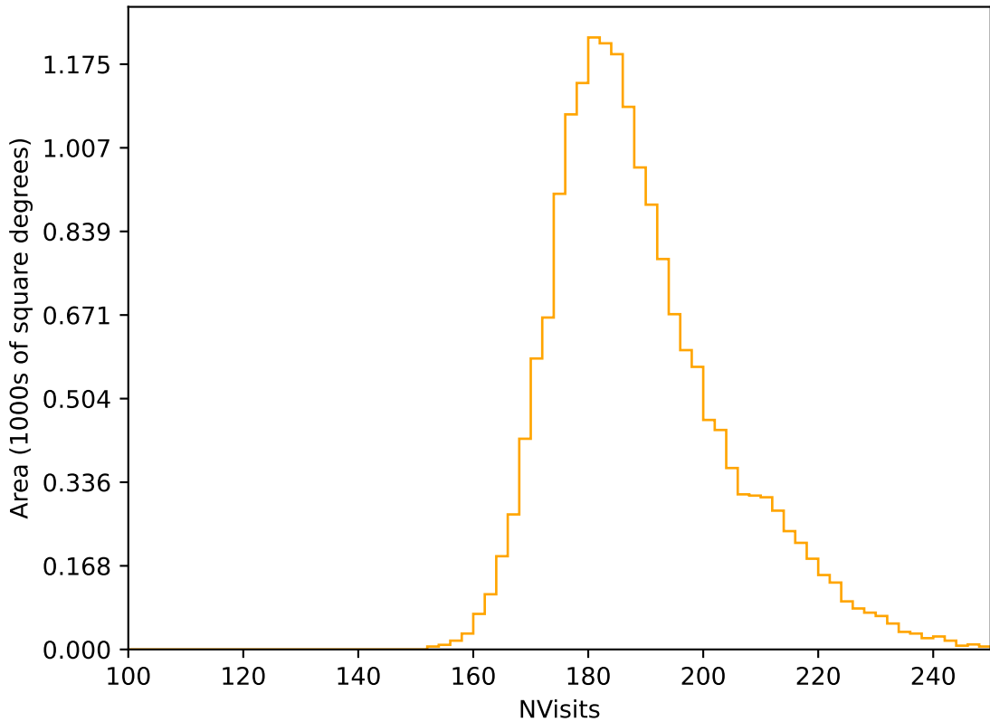
too_elab_r32_d2_giz_v3.4_10yrs WFD r band: NVisits
