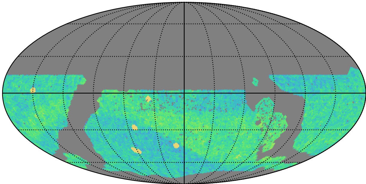
too_elab_r32_d2_giz_v3.4_10yrs WFD i band: NVisits
