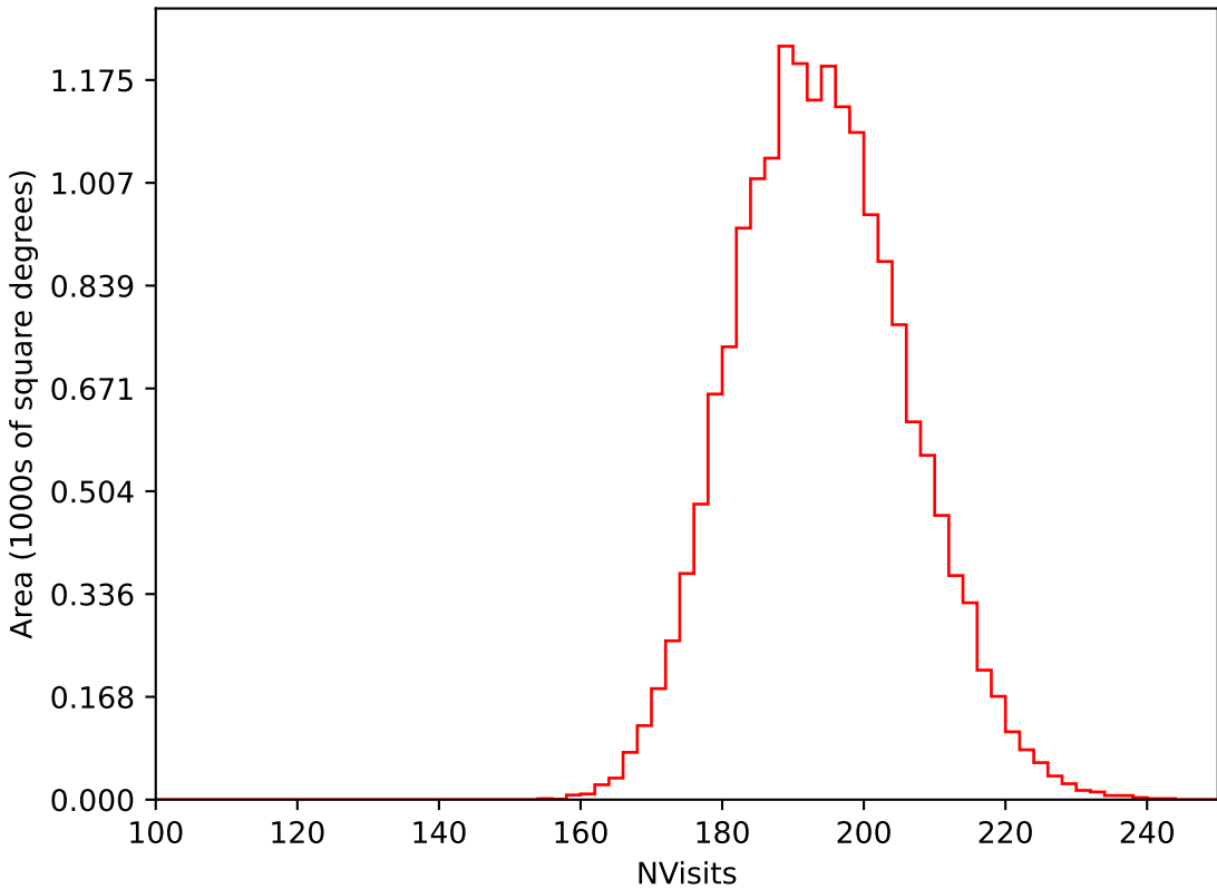
too_elab_r32_d2_giz_v3.4_10yrs WFD i band: NVisits
