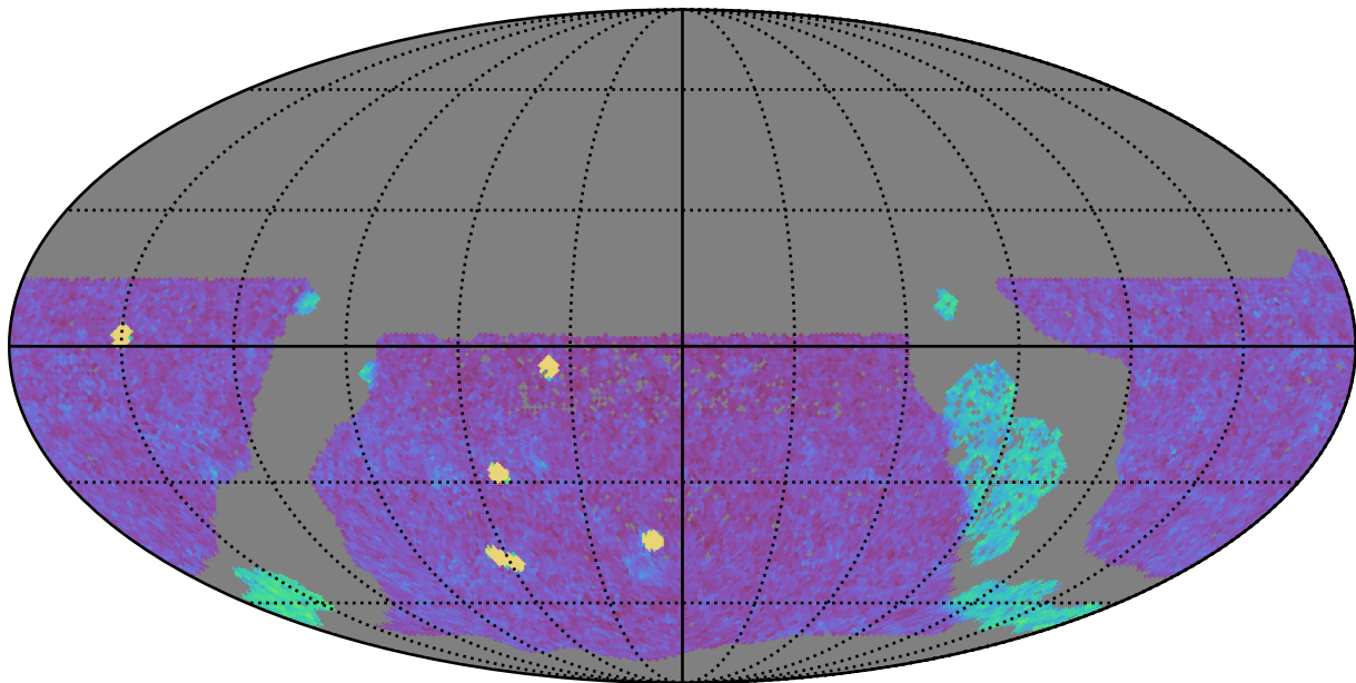
too_elab_r32_d2_giz_v3.4_10yrs WFD g band: NVisits
