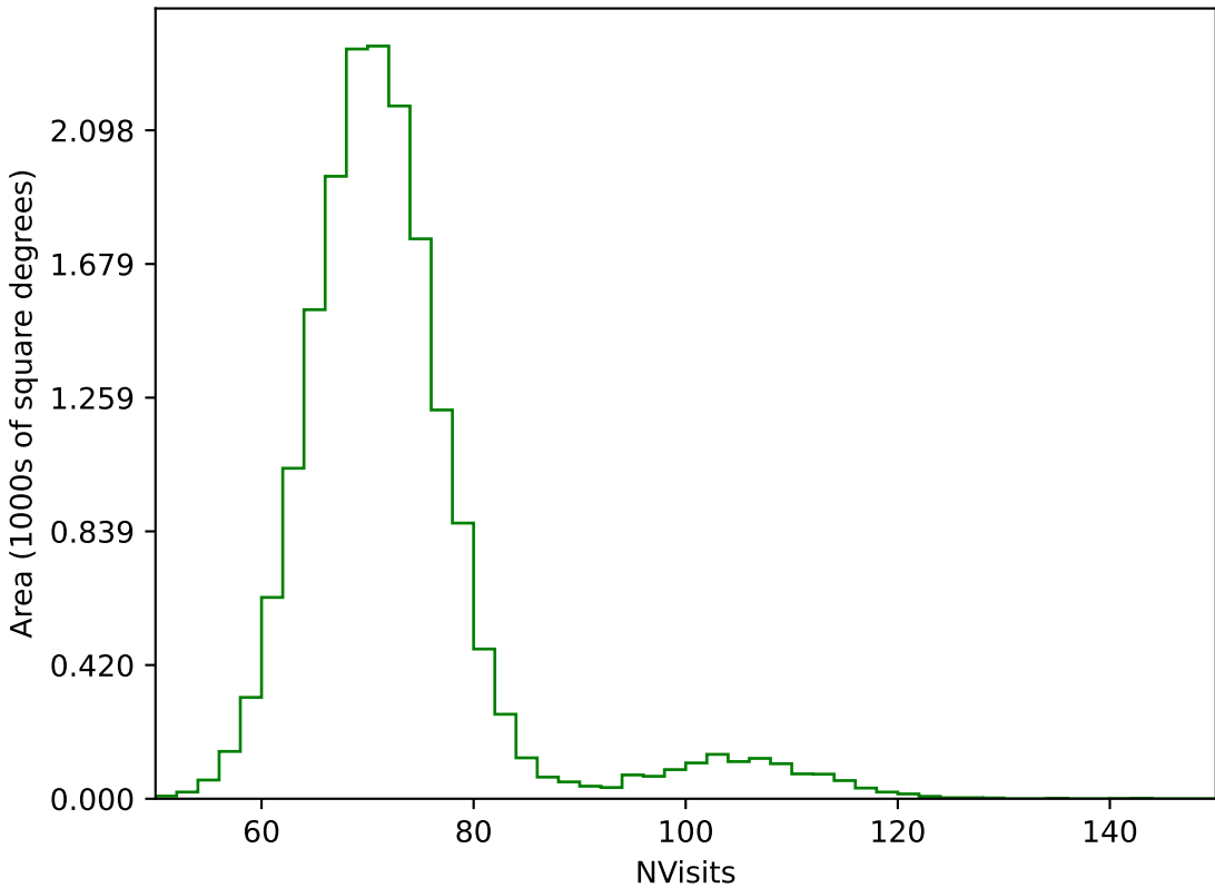
too_elab_r32_d2_giz_v3.4_10yrs WFD g band: NVisits
