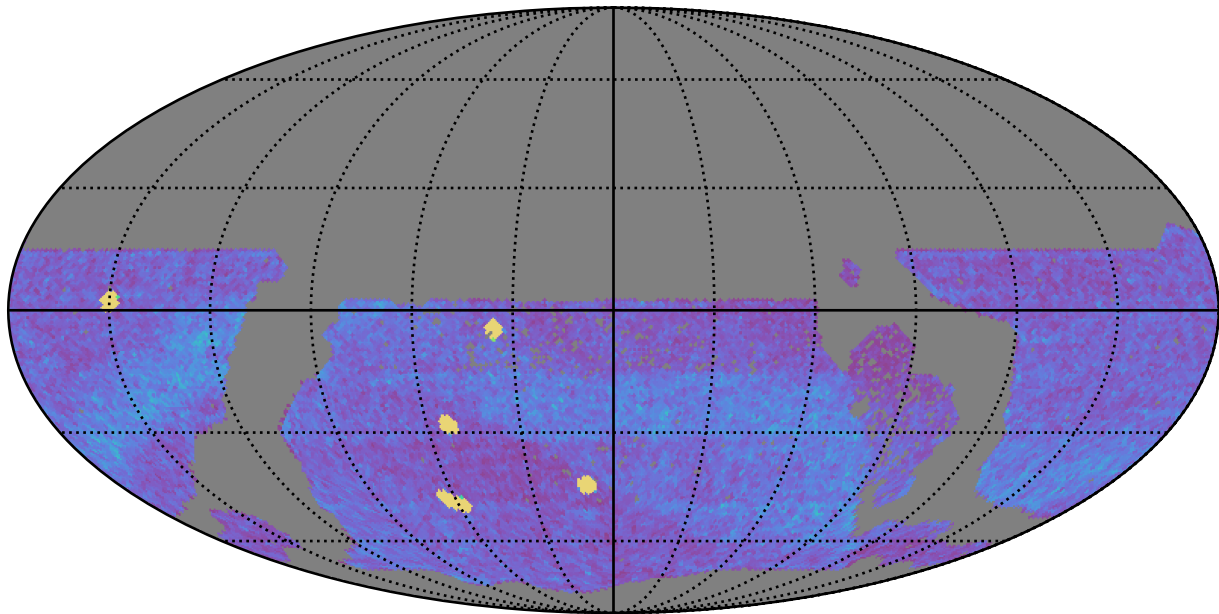
too_elab_r32_d2_giz_v3.4_10yrs WFD all bands: NVisits
