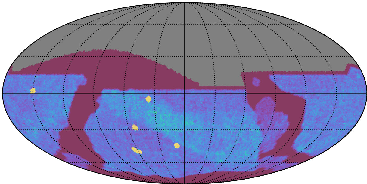
too_elab_r32_d2_giz_v3.4_10yrs All sky z band: NVisits
