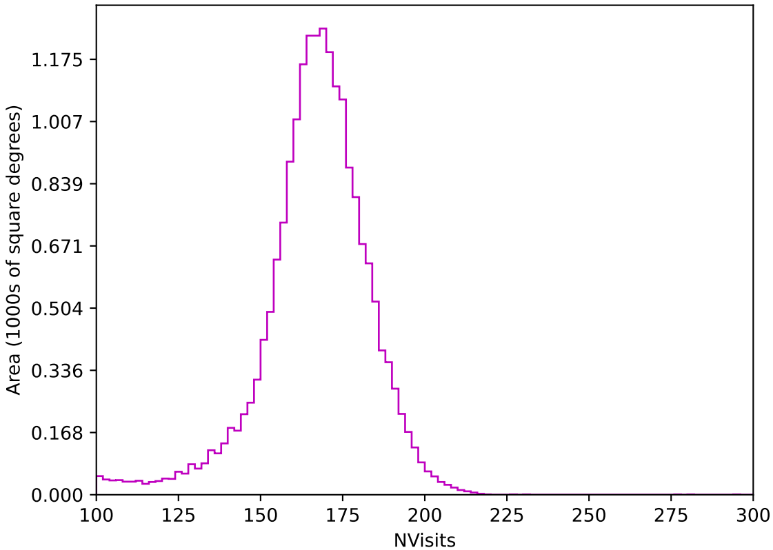
too_elab_r32_d2_giz_v3.4_10yrs All sky z band: NVisits
