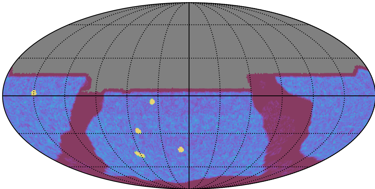
too_elab_r32_d2_giz_v3.4_10yrs All sky y band: NVisits
