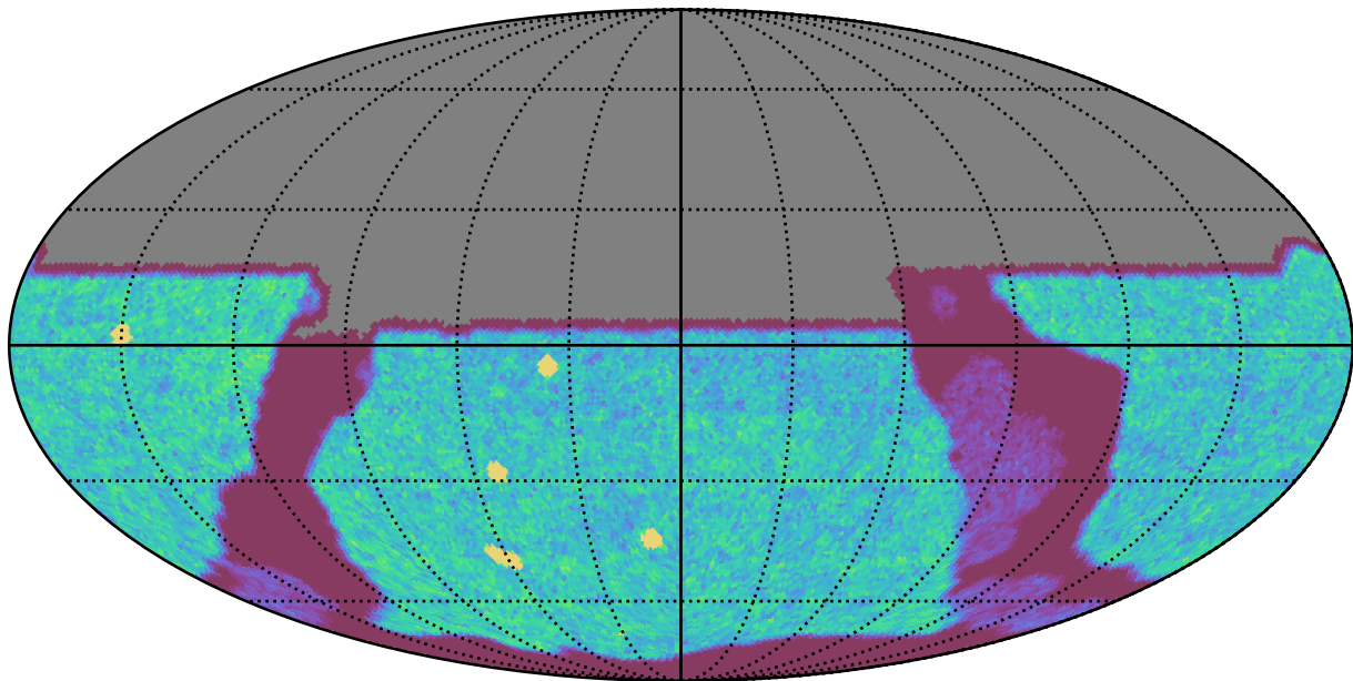
too_elab_r32_d2_giz_v3.4_10yrs All sky u band: NVisits
