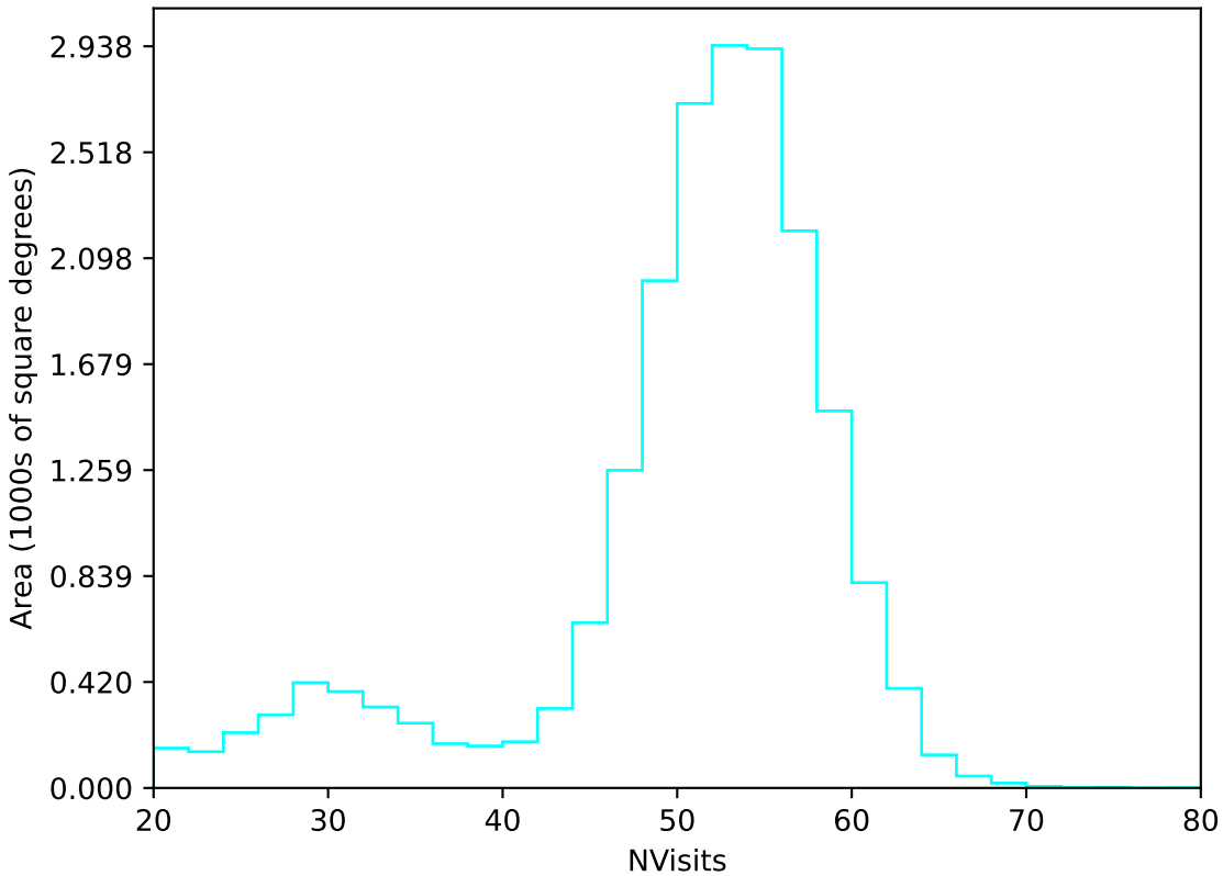
too_elab_r32_d2_giz_v3.4_10yrs All sky u band: NVisits
