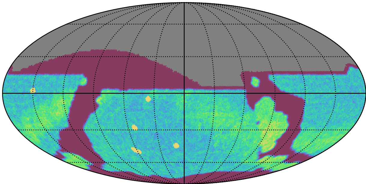
too_elab_r32_d2_giz_v3.4_10yrs All sky r band: NVisits
