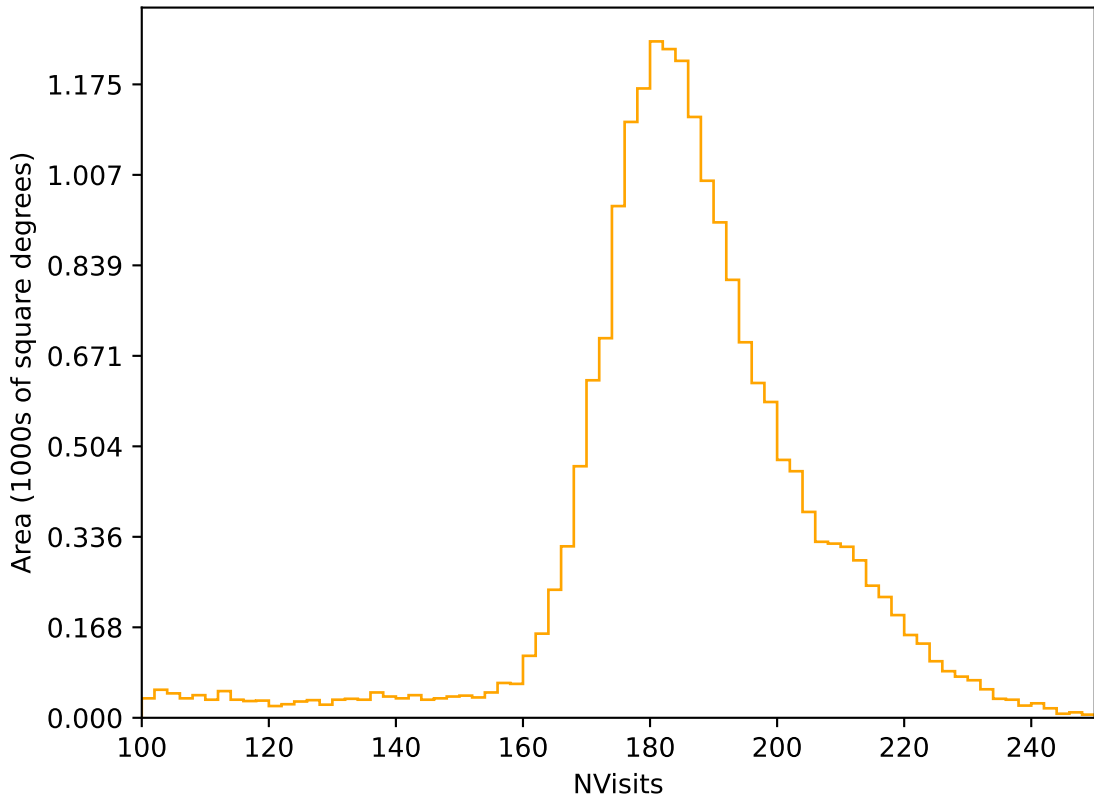
too_elab_r32_d2_giz_v3.4_10yrs All sky r band: NVisits
