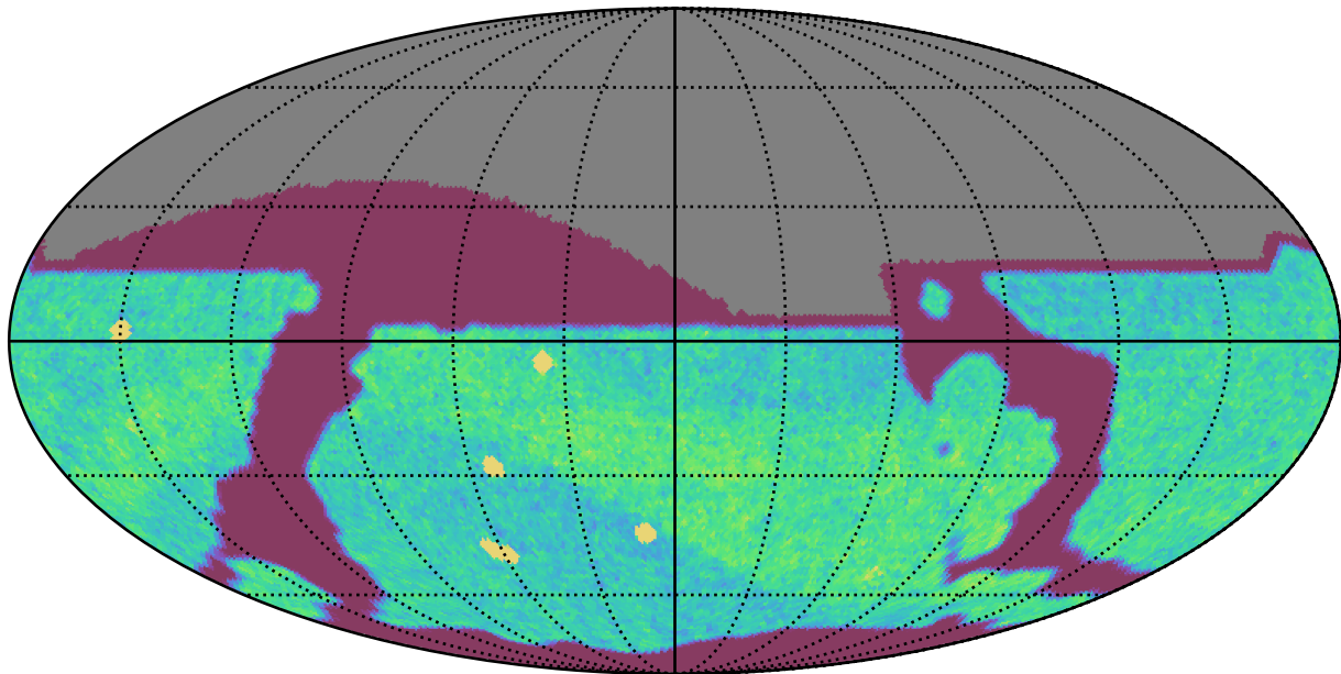
too_elab_r32_d2_giz_v3.4_10yrs All sky i band: NVisits
