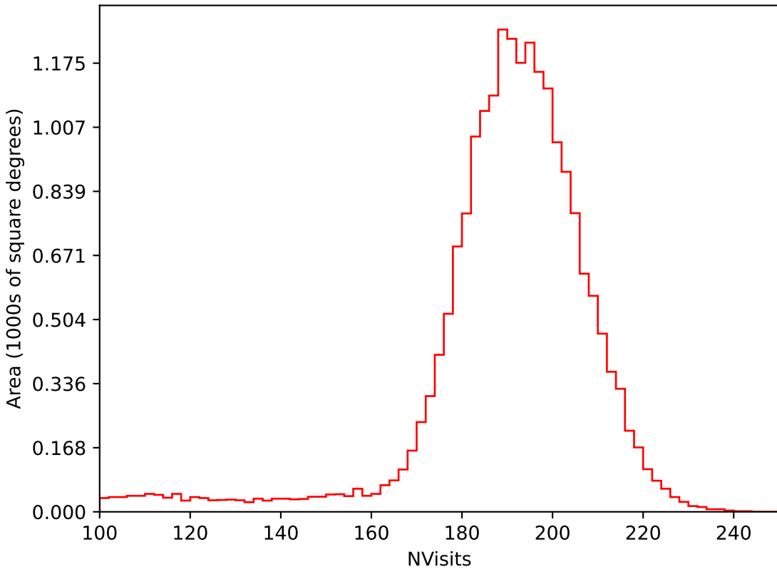
too_elab_r32_d2_giz_v3.4_10yrs All sky i band: NVisits
