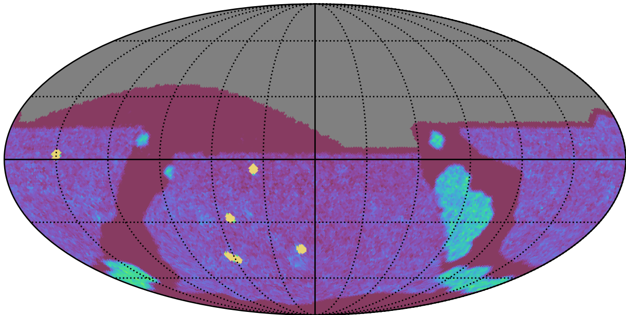
too_elab_r32_d2_giz_v3.4_10yrs All sky g band: NVisits
