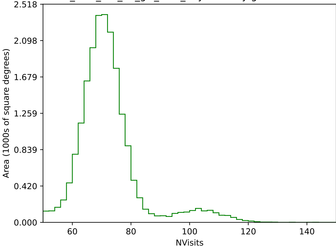
too_elab_r32_d2_giz_v3.4_10yrs All sky g band: NVisits
