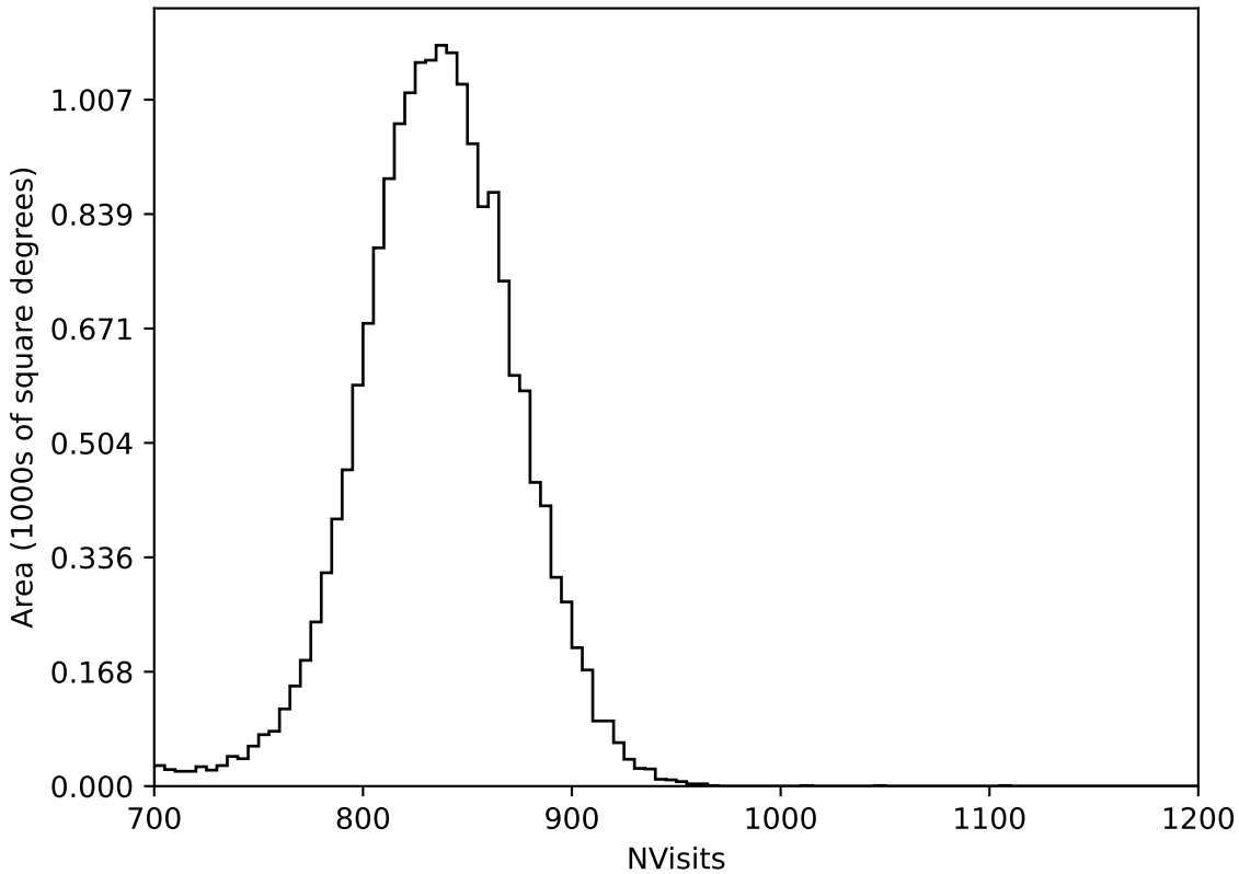
too_elab_r32_d2_giz_v3.4_10yrs All sky all bands: NVisits
