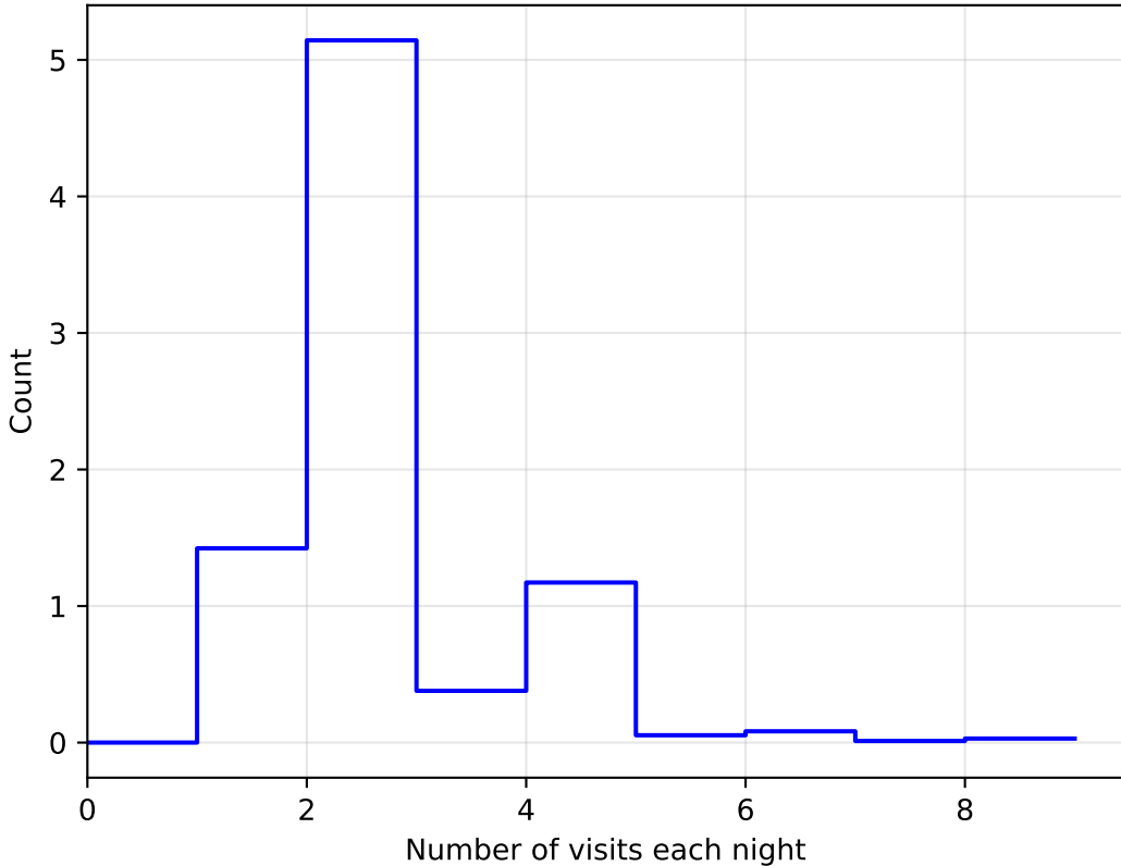
too_elab_r32_d2_giz_v3.4_10yrs WFD: NVisitsPerNight
