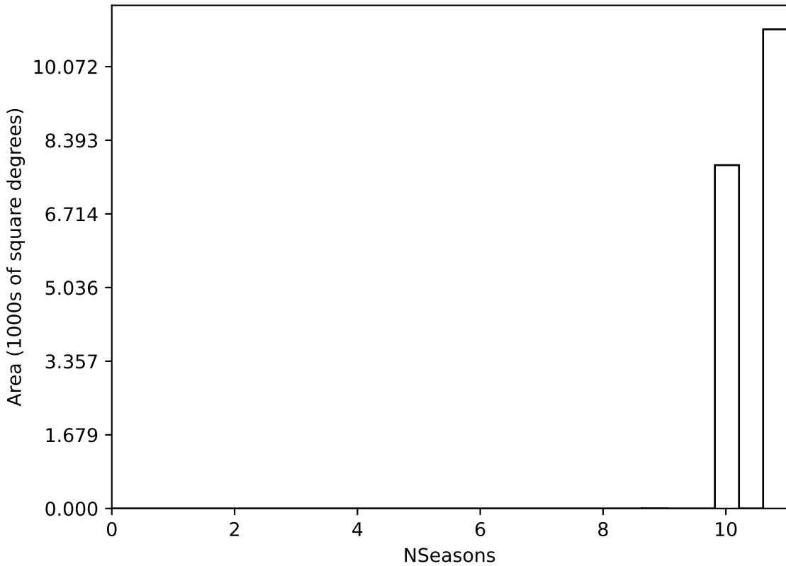
too_elab_r32_d2_giz_v3.4_10yrs WFD all bands: NSeasons
