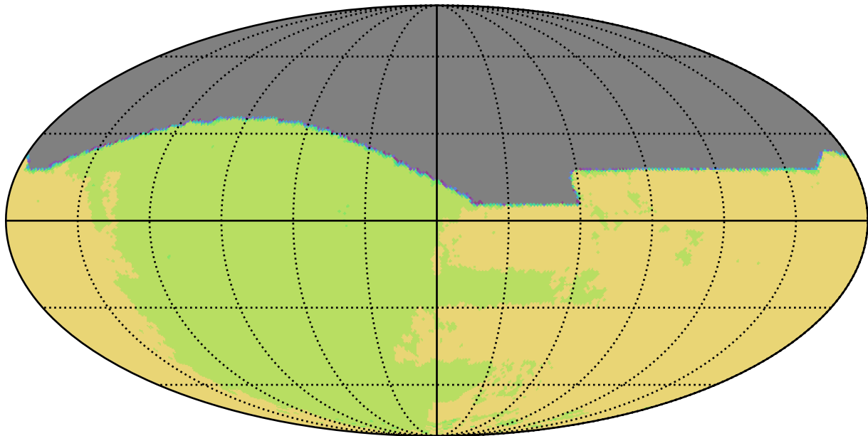
too_elab_r32_d2_giz_v3.4_10yrs All sky all bands: NSeasons
