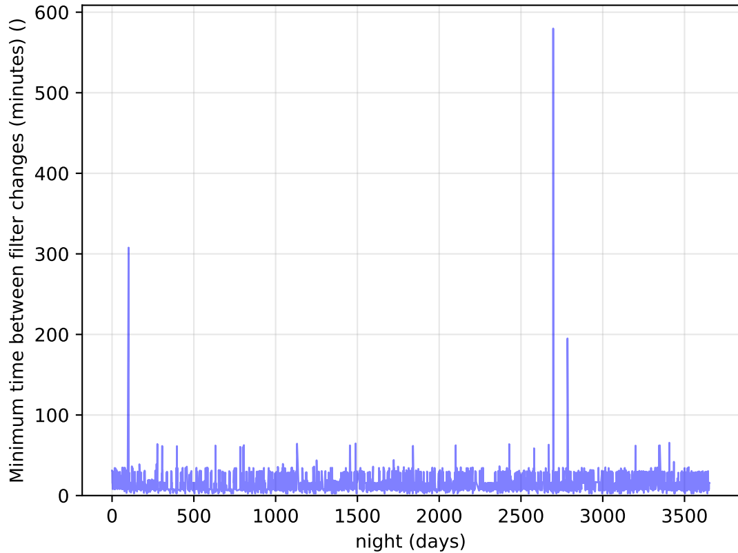
too_elab_r32_d2_giz_v3.4_10yrs Per Night: Minimum time between filter changes (minutes)
