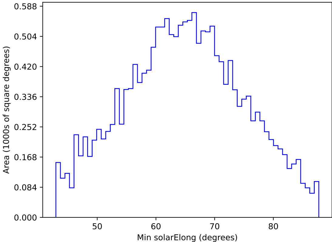
too_elab_r32_d2_giz_v3.4_10yrs WFD y band: Min solarElong
