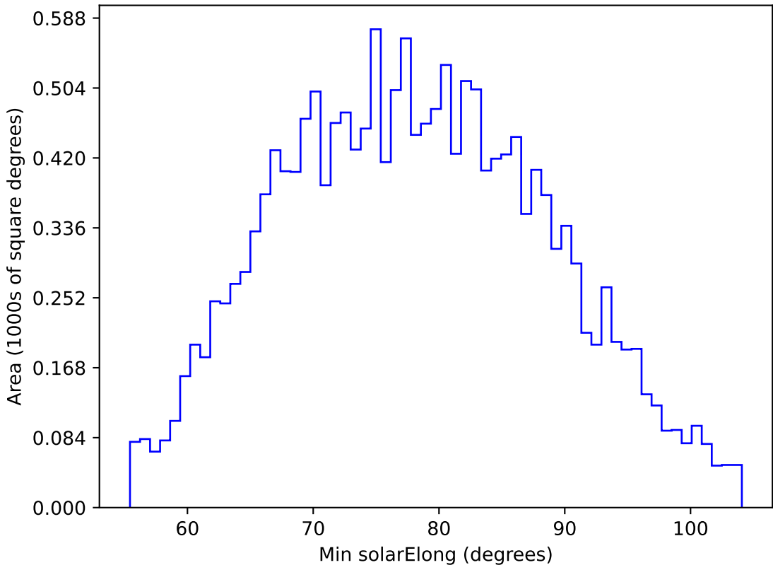
too_elab_r32_d2_giz_v3.4_10yrs WFD u band: Min solarElong
