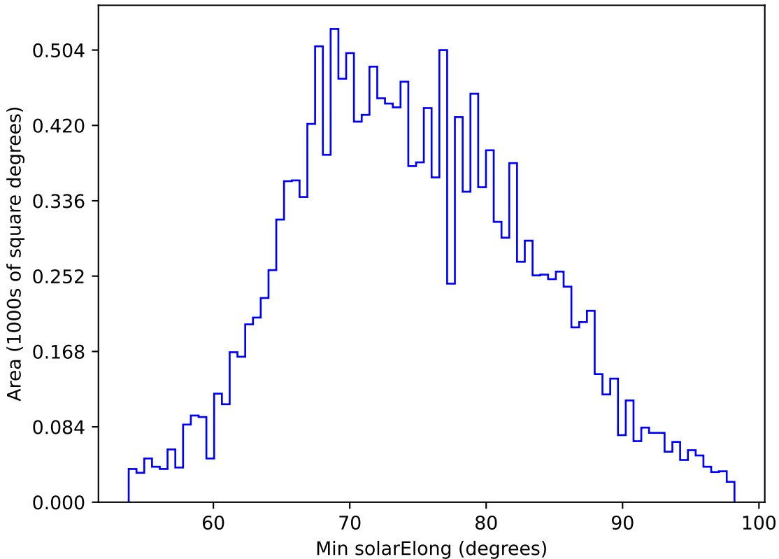
too_elab_r32_d2_giz_v3.4_10yrs WFD g band: Min solarElong
