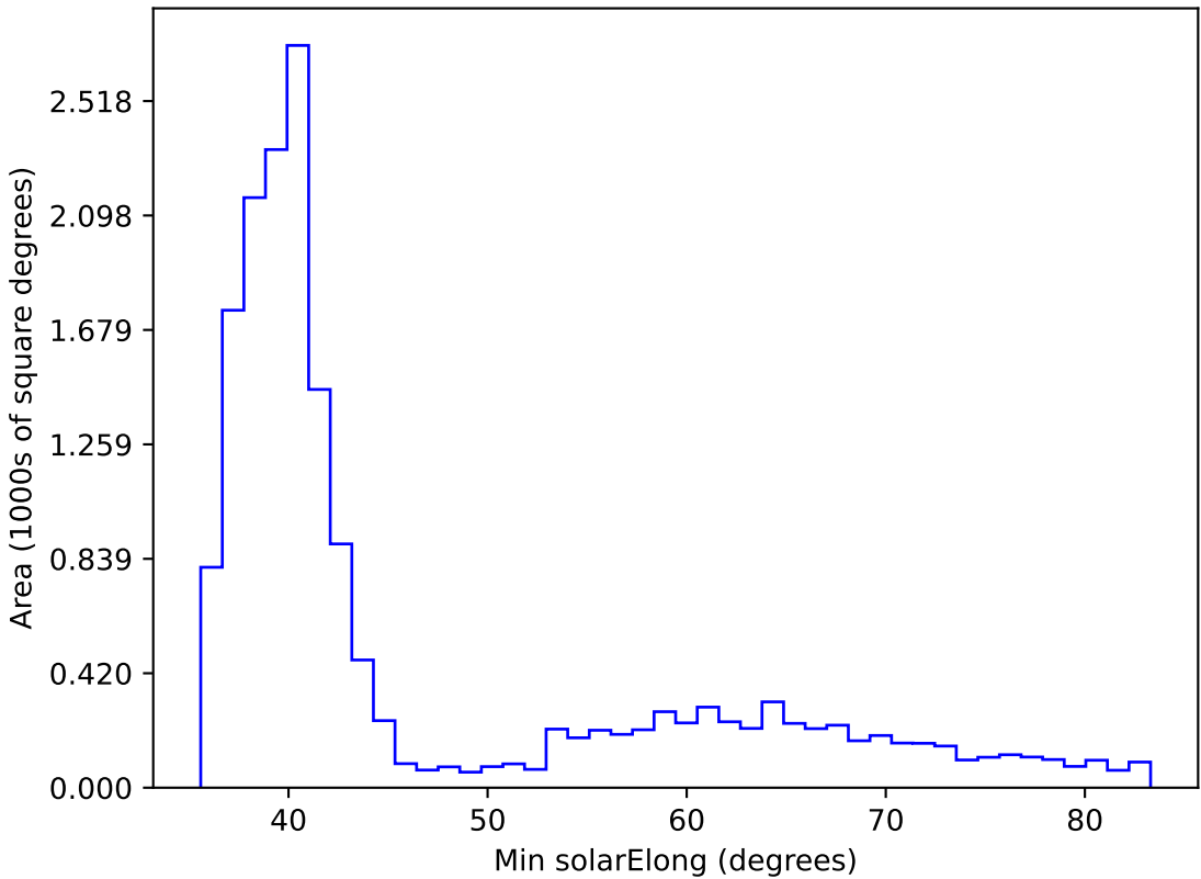
too_elab_r32_d2_giz_v3.4_10yrs WFD all bands: Min solarElong
