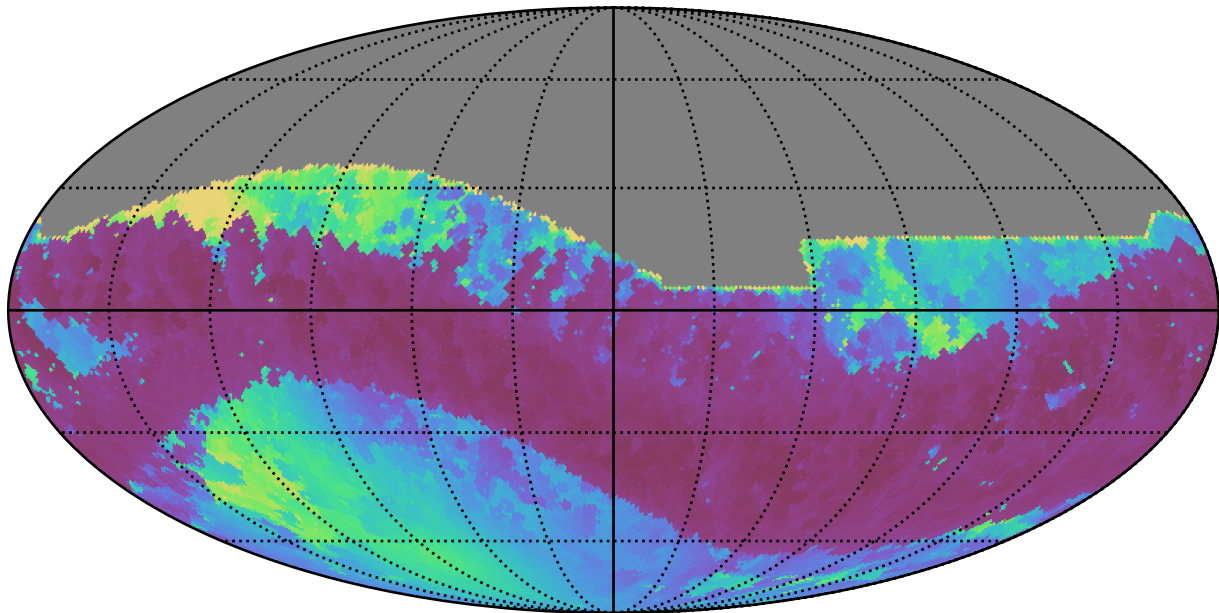
too_elab_r32_d2_giz_v3.4_10yrs All sky z band: Min solarElong
