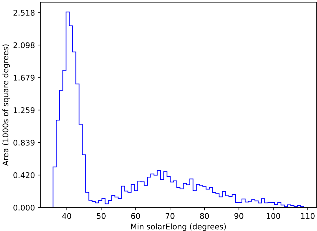
too_elab_r32_d2_giz_v3.4_10yrs All sky z band: Min solarElong
