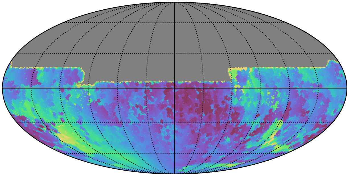
too_elab_r32_d2_giz_v3.4_10yrs All sky y band: Min solarElong
