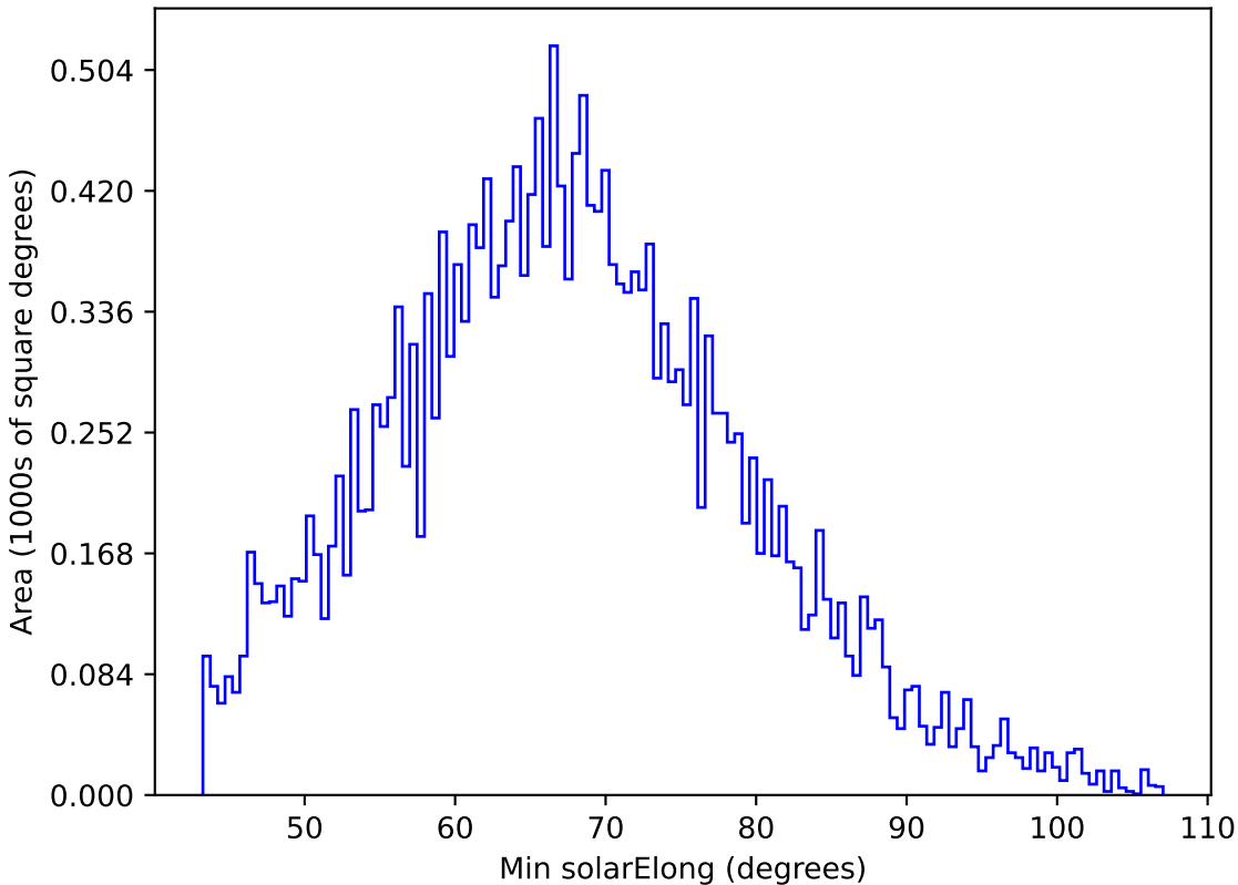
too_elab_r32_d2_giz_v3.4_10yrs All sky y band: Min solarElong
