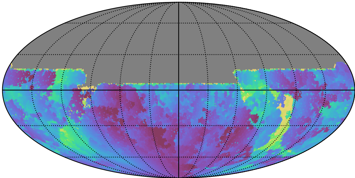
too_elab_r32_d2_giz_v3.4_10yrs All sky u band: Min solarElong
